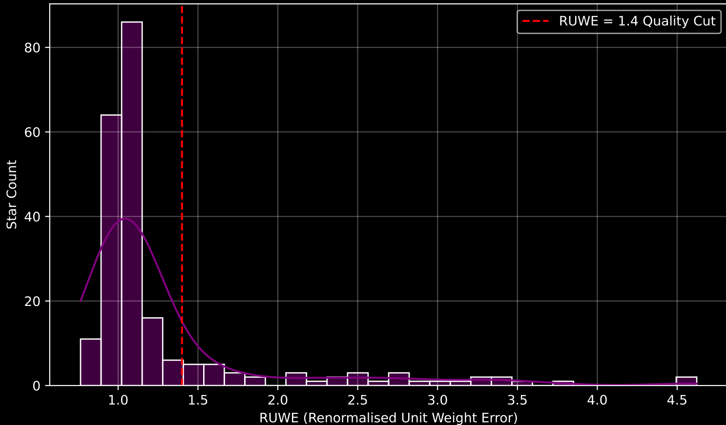
GAPOGEE DR17 Field [266+56-O] RUWE Distribution (n= 222)
