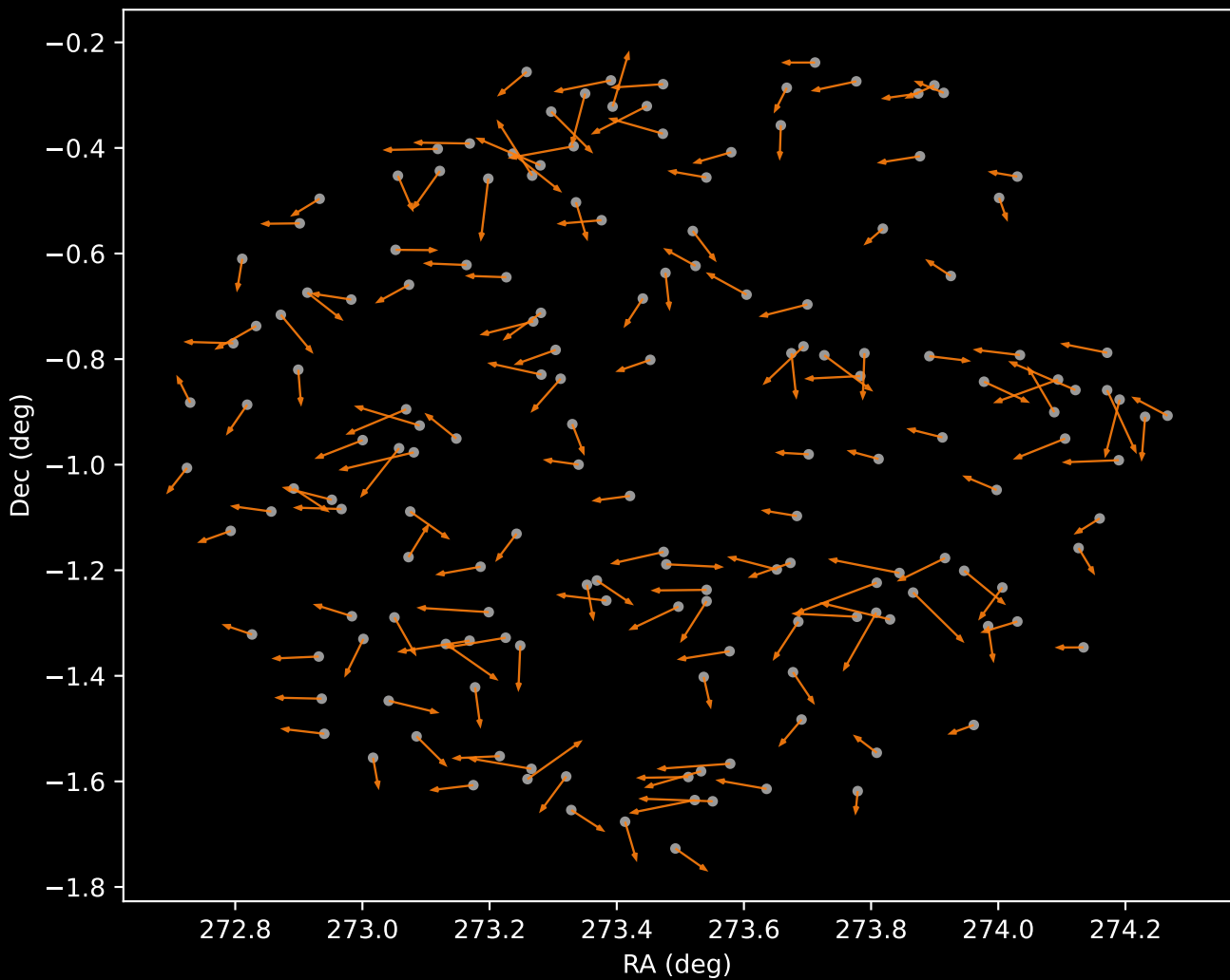
APOGEE DR17 Cluster 2 Proper Motion Vectors (n=164)
