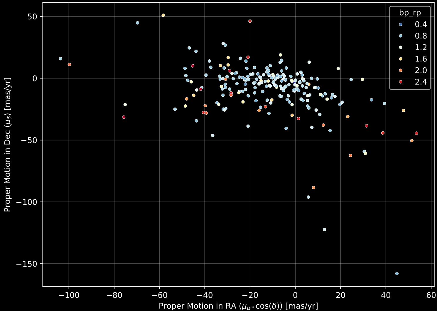
APOGEE DR17 Field: [266+56-O] Proper Motion Diagram (n= 232)
