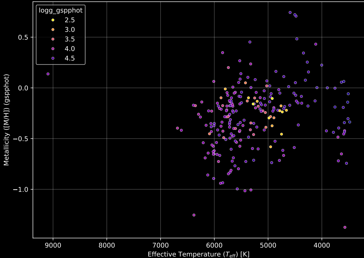
APOGEE DR17 Field: [266+56-O] Stellar Population Parameters (n= 232)
