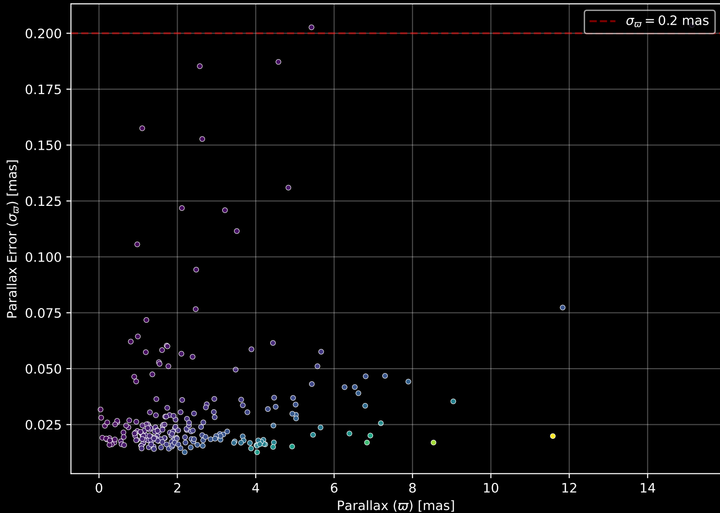
APOGEE DR17 Field: [266+56-O] Parallax Quality (n= 232)
