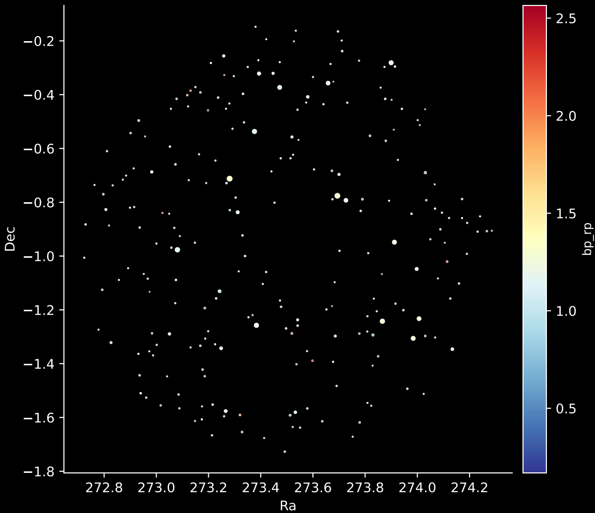
APOGEE DR17 Field: [266+56-O] Stars: 232
