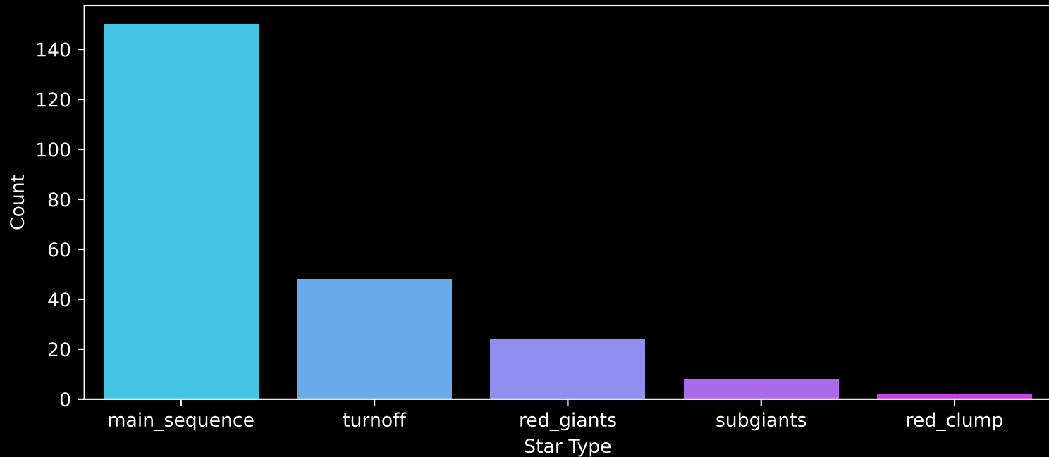
APOGEE DR17 Field: [266+56-O] Count plot of Star Type
